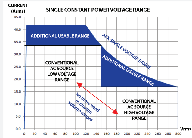
3150AFX (15kVA) operating at a constant 5 kVA per phase. The blue-shaded area shows expanded range compared to conventional 150V/300V sources.
