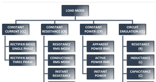
Available ELZ Load Operating Modes
