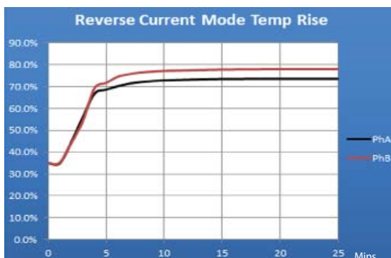
Figure 8: Reverse Current Mode Temperature Rise
