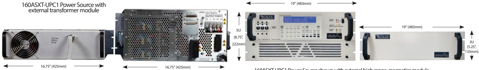
160ASXT-UPC1 Power Source shown with external high range magnetics module.
