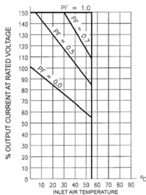
THERMAL DERATING CHART
